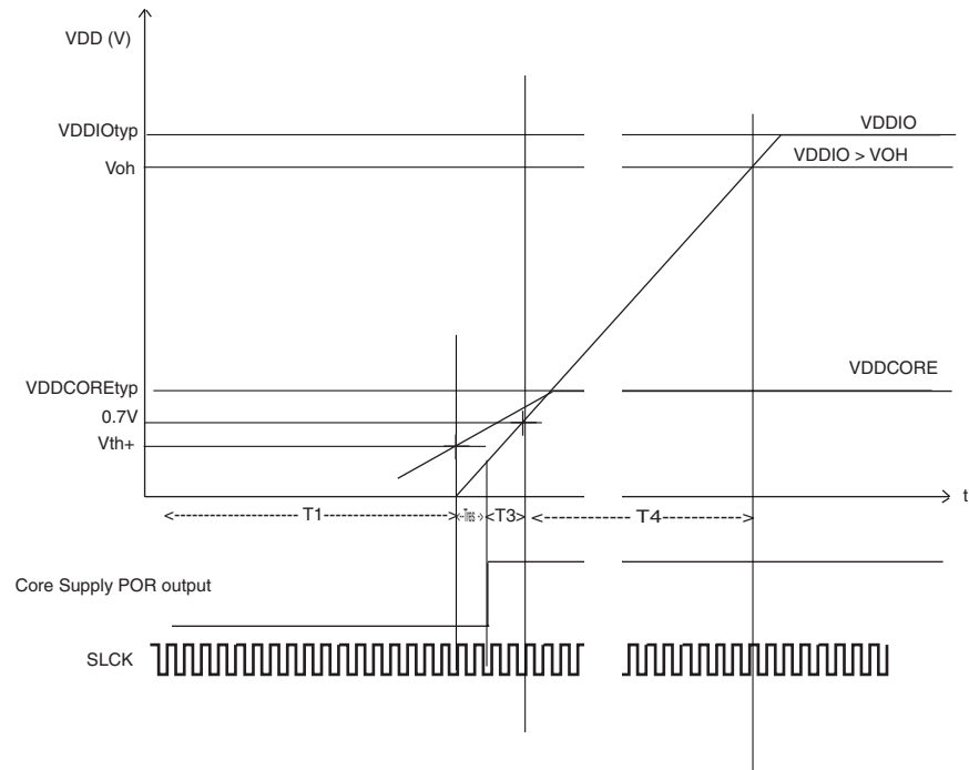
Figure 4-2. V_{VDDCORE} and V_{VDDIO} Constraints at Power-up
