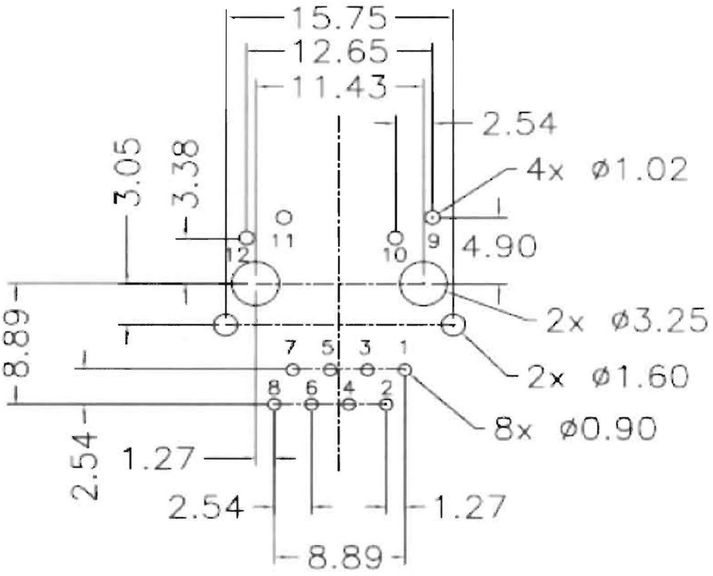
RECOMMENDED P.C.PATTERN.COMPONENT SIDE
