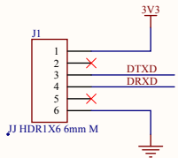
DPI interface - console port
